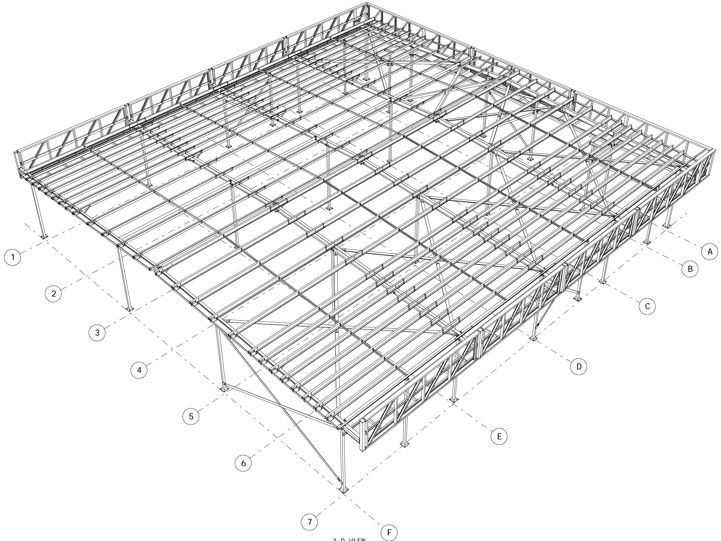
3-D VIEW
